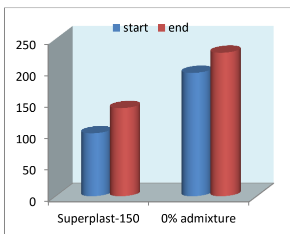
Rys.1. Setting time in temp. 20°C [min]
